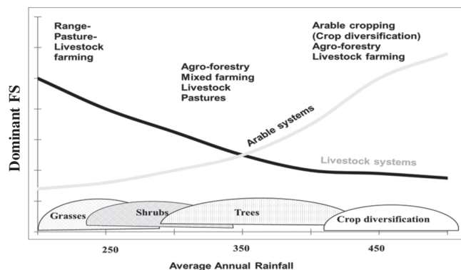
Fig. 1. Dominance of various farming systems according to rainfall pattern in arid zone
